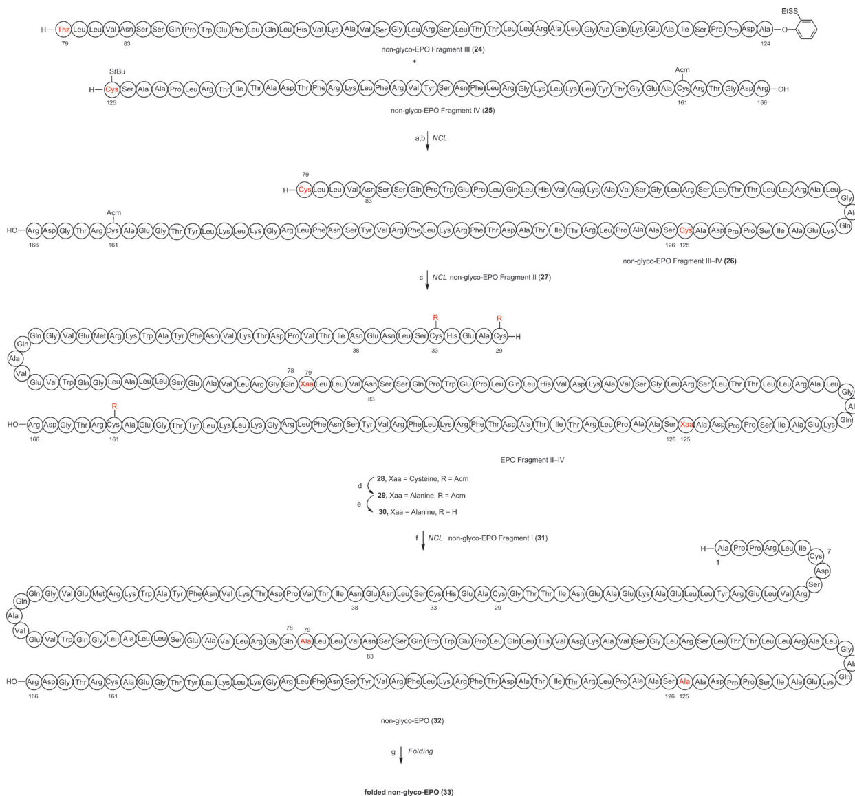
Scheme 9. Synthesis of non-glyco-EPO. Reaction conditions: a) Gn-HCl (6 mM), Na 2 HPO 4 (0.2 mM), TCEP-HCl (0.02 mM), MPAA (0.2 mM), Bond-Breaker reducing agent, pH 7.2–7.4; b) MeONH 2 -HCl (0.3 mM), pH 4.0, 34 % yield over 2 steps; c) Gn-HCl (6 mM), Na 2 HPO 4 (0.2 mM), TCEP-HCl (0.02 mM), MPAA (0.2 mM), Bond-Breaker reducing agent, pH 7.2–7.4; 33 % yield; d) Gn-HCl (6 mM), Na 2 HPO 4 (0.2 mM), TCEP-HCl (0.08 mM) pH 7.0, VA-044, tBuSH, 37°C; e) AgOAc, CH 3 CN/H 2 O (1:1) + 0.05 % TFA then DTT, 45 % yield over 2 steps; f) Gn-HCl (6 mM), Na 2 HPO 4 (0.2 mM), TCEP-HCl (0.02 mM), MPAA (0.2 mM), Bond-Breaker reducing agent, pH 7.2–7.4, 35–40 % yield; g) Tris-HCl (50 mM), CuSO 4 (40 mM), N -lauroylsarcosine (2 % w/v), pH 8.0.
